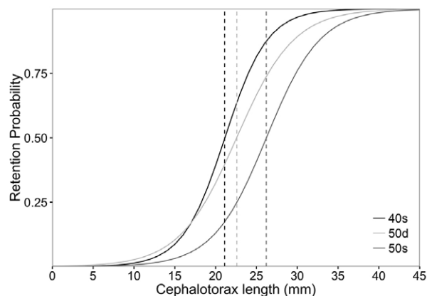
Fig. 5. – Mean selectivity curves for the 50-mm diamond mesh (50d), 40-mm square mesh (40s) and 50-mm square mesh (50s), obtained taking into account between-haul variability. The vertical dashed lines indicate the L 50 for the three mesh configurations (black, 40s; light grey, 50d; dark grey, 50s).
