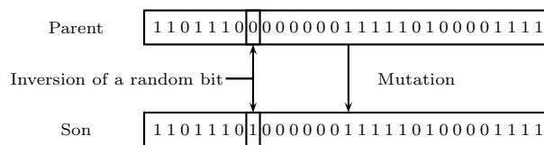
Figure 4.11: Diagram showing an example of the generation of a new entity by mutation.
