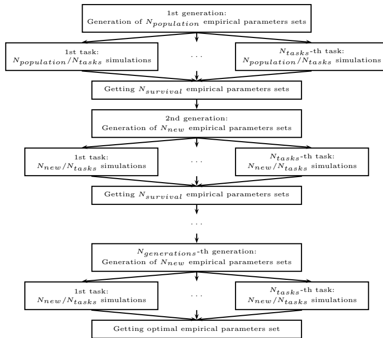
Figure 4.14: Flowchart of the parallelization scheme implemented in Genetic for the genetic method.
