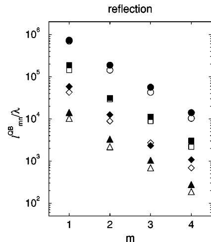
FIG. 9. Same as Fig. 3 but in reflection.
