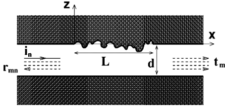
FIG. 1. Illustration of the waveguide geometry.
