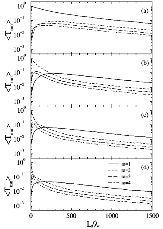
FIG. 4. Same as in Fig. 2 but for \delta/\lambda = 0.1 .
