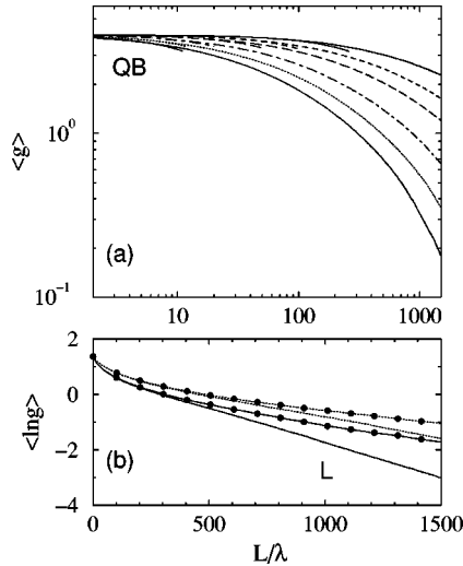
FIG. 13. (a) Mean dimensionless conductance as a function of the length L in a log-log plot for a waveguide width d/\lambda=2.25 , supporting four modes, with disorder parameters a/\lambda=0.2 and \delta/\lambda=0.02 (upper solid curve), 0.03 (dashed curve), 0.04 (long dashed curve), 0.06 (dot-dashed curve), 0.08 (dotted curve), and 0.1 (lower solid curve). Averages over N_p=4000 realizations. Fits to the QB regimes are shown. (b) \langle \ln g \rangle (without dots) and \ln \langle g \rangle (with dots) for \delta/\lambda=0.08 (dotted curves) and 0.1 (solid curves), revealing the L regimes.
