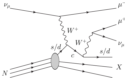
Fig. 1. Feynman diagram of a \nu_\mu induced Charged Current charm dimuon event.
