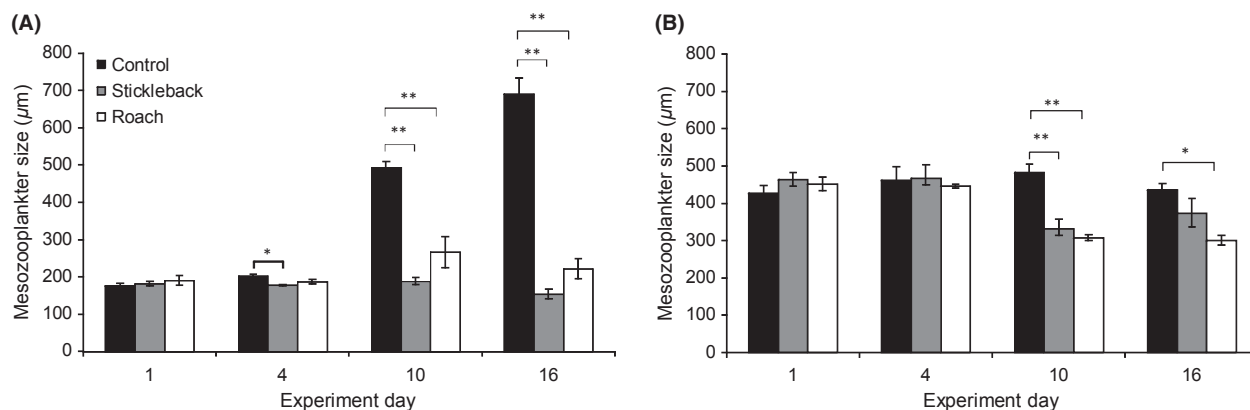
Figure 2. Mean weighted size of the average mesozooplankter (rotifers and crustaceans) in spring (A) and summer (B) experiments. Asterisks indicate significant differences (* P < 0.05 , ** P < 0.01 ) between treatments. Error bars are \pm SE.
