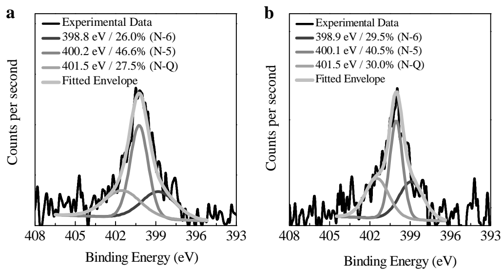
Figure S1. N 1s XPS spectra of AG650 (a) and AG700 (b).
