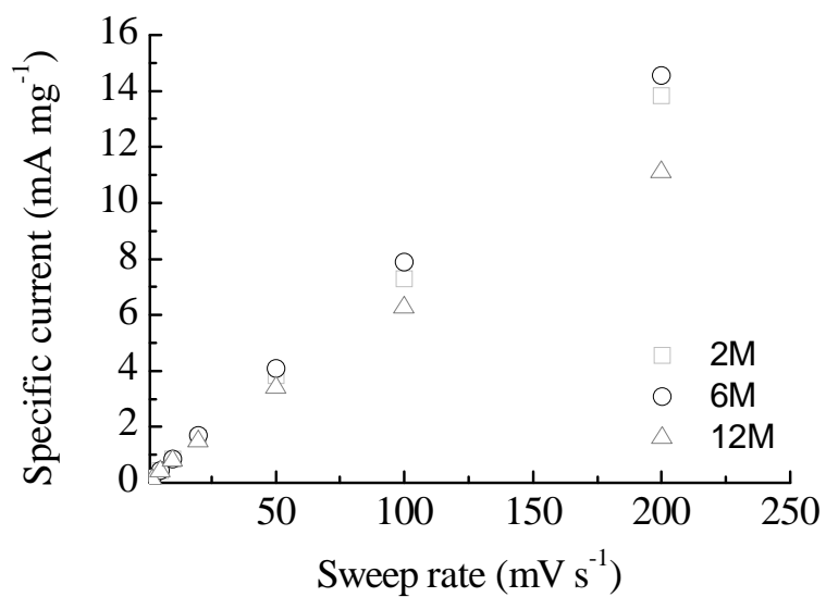
Figure S3. Sweep rate dependency of the specific current at 0 V in LiCl electrolyte of different concentrations (Sample: AG700).
