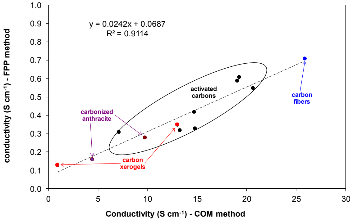
Figure 2. Correlation between the electrical conductivity measured by four-point probing (FPP) and compression (COM) for the materials with moderate conductivity.
