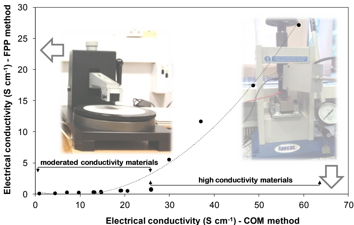
Figure 1. Relationship between the electrical conductivity measured by four-point probe (FPP) and compression (COM) for the series of materials studied.
