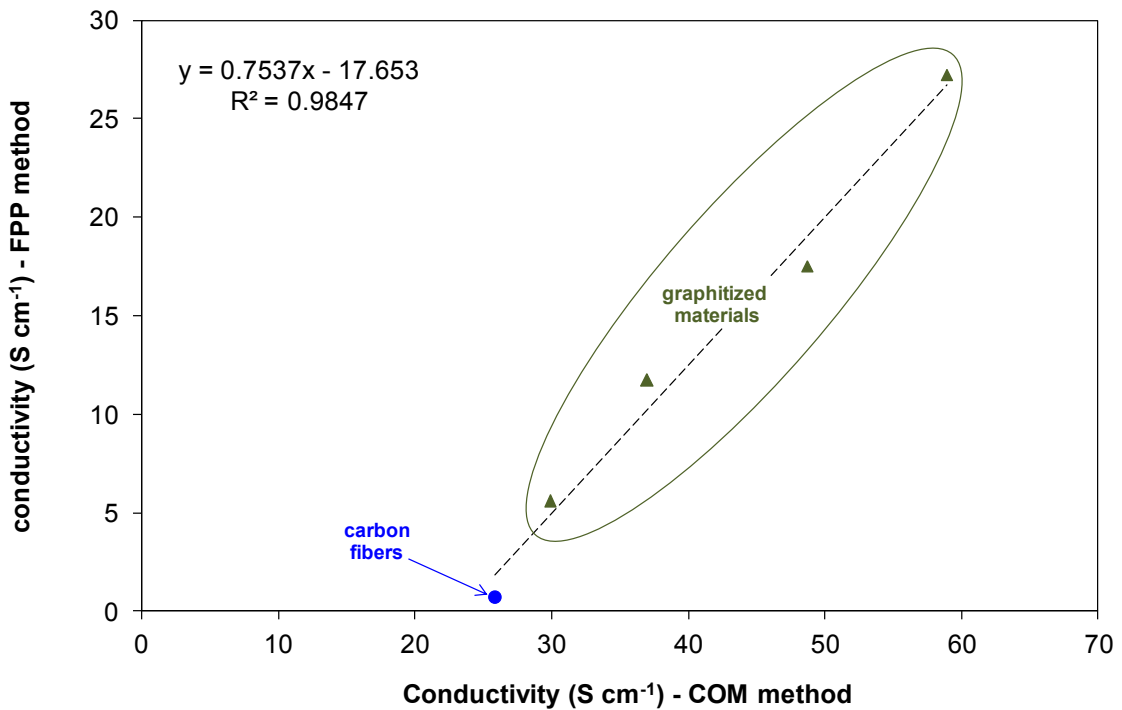
Figure 3. Correlation between the electrical conductivity measured by four-point probing (FPP) and compression (COM) for the materials with a high conductivity.
